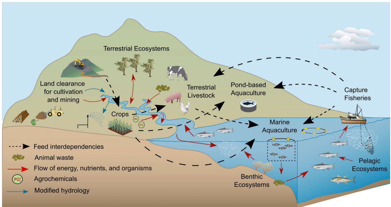
FIGURE 4 Feed interdependencies redistribute land-sea nutrient flows over large spatial scales. Run-off from land-clearance and agricultural nutrient waste influences the productivity of coastal waters globally, while fisheries may disrupt the flow of nutrients to terrestrial ecosystems. The trade, use, and waste of livestock and aquaculture feeds redistribute nutrients between land and sea, often over vast distances. Intensified use of feed products then contributes to aquatic and terrestrial nutrient surpluses, interacting with natural land-sea connectivity
